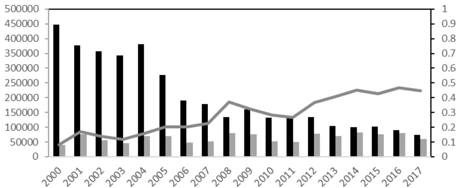
Commercial and total recreational salmon catches (SD 22 - 32)
